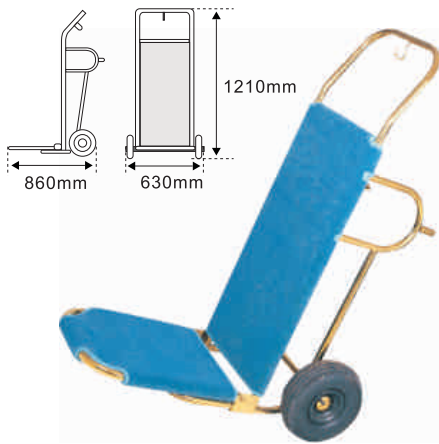
Item# BC1.2222 Size 630 X 860 x (H)1210mm
